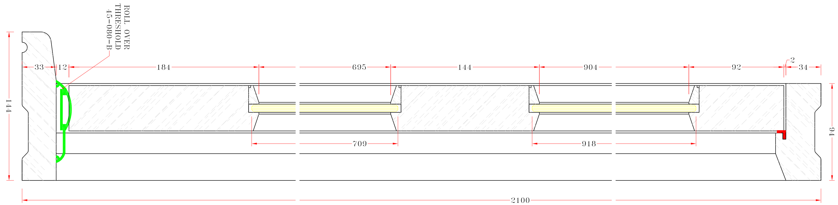
1:2 HEIGHT SECTION THRU 'DD'
